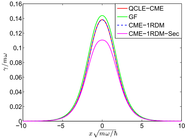
FIG. 2. Electronic friction as a function of x for model #2 where the system Hamiltonian is diagonal. Results from the QCLE-CME (Eq. (26)) and CME-1RDM (Eq. (49)) agree exactly and closely match the Green's function (GF) results (though without broadening). CME-1RDM-Sec results (Eq. (51)) perform less well, highlighting the limitations of the secular approximation, which ignores off-diagonal contributions to the electronic friction (as caused by intramolecular coherence). kT = 0.01 , \hbar\omega = 0.003 , g = 0.0075 , \Delta = 0.01 , V = 0 , \Gamma = 0.01 .
