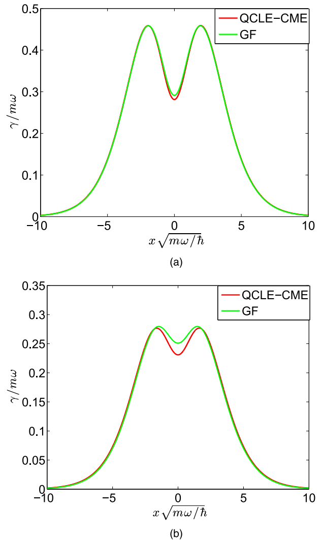
FIG. 1. Electronic friction as a function of x for model #1, with a non-diagonal \hat{H}_s^{el} . (a) In the Redfield regime (small \Gamma ), our QCLE-CME result (Eq. (26)) agrees with the Green's function (GF) result (Eq. (58)) very well. (b) For larger \Gamma , the QCLE-CME and GF results agree less well, where we find that usually the QCLE-CME result has sharper dips or peaks due to a lack of broadening. kT = 0.01 , \hbar\omega = 0.003 , g = 0.0075 , V = 0.01 . (a) \Gamma = 0.01 . (b) \Gamma = 0.02 .
