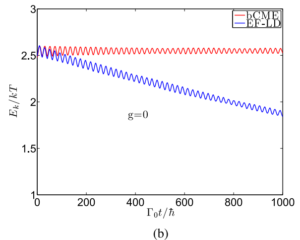
FIG. 4. Average kinetic energy as a function of time for the generalized AH model in Eqs. (1)-(4): K = 1 , \hbar\omega = 0.003 , \Gamma_0 = 0.02 , kT = 0.01 , \bar{E}_d = 0 , \mu = 0 , W = 1 . See Eqs. (73)-(75) for definition of the parameters. (a) For g = 0.0075 , we get good agreement between bCME and EF-LD, even though the bCME friction (Eq. (59)) is different from total EF-LD friction (Eq. (72)). (b) However, the bCME does fail when \partial_x h is very small. Here, \partial_x h = \sqrt{2}g = 0 so that the kinetic energy does not relax at all according to the bCME.
